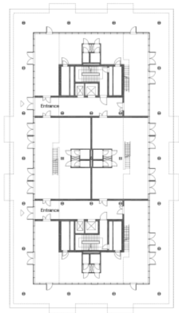
Groundfloor plan
